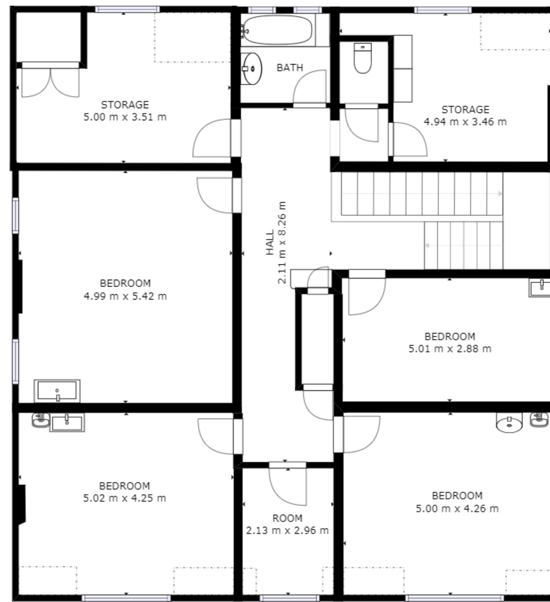
FLOOR 3
